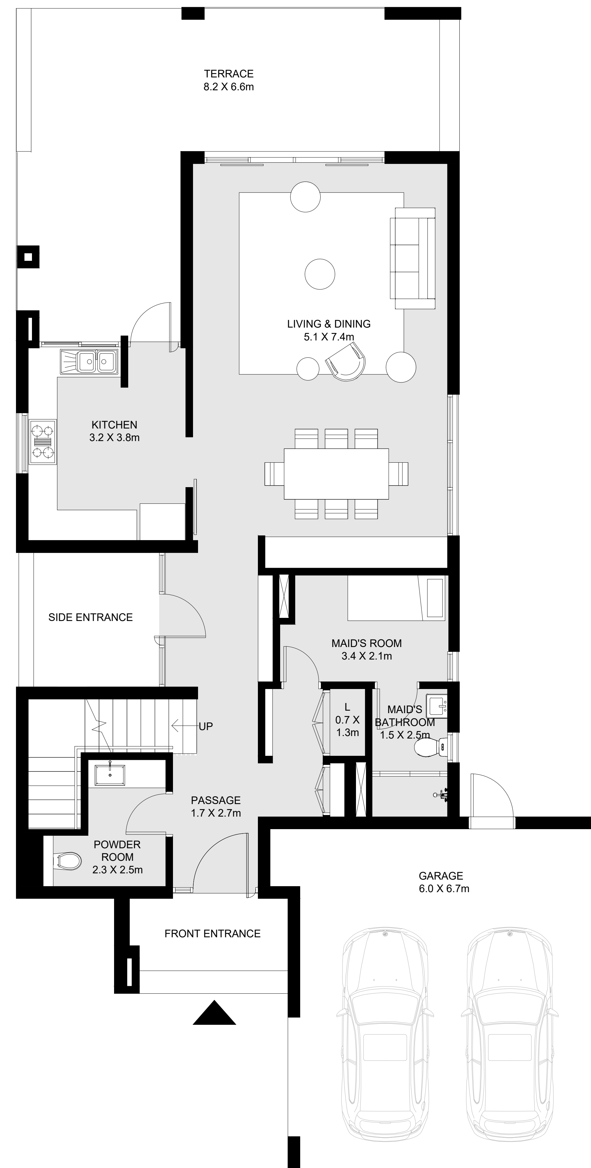
GROUND FLOOR
