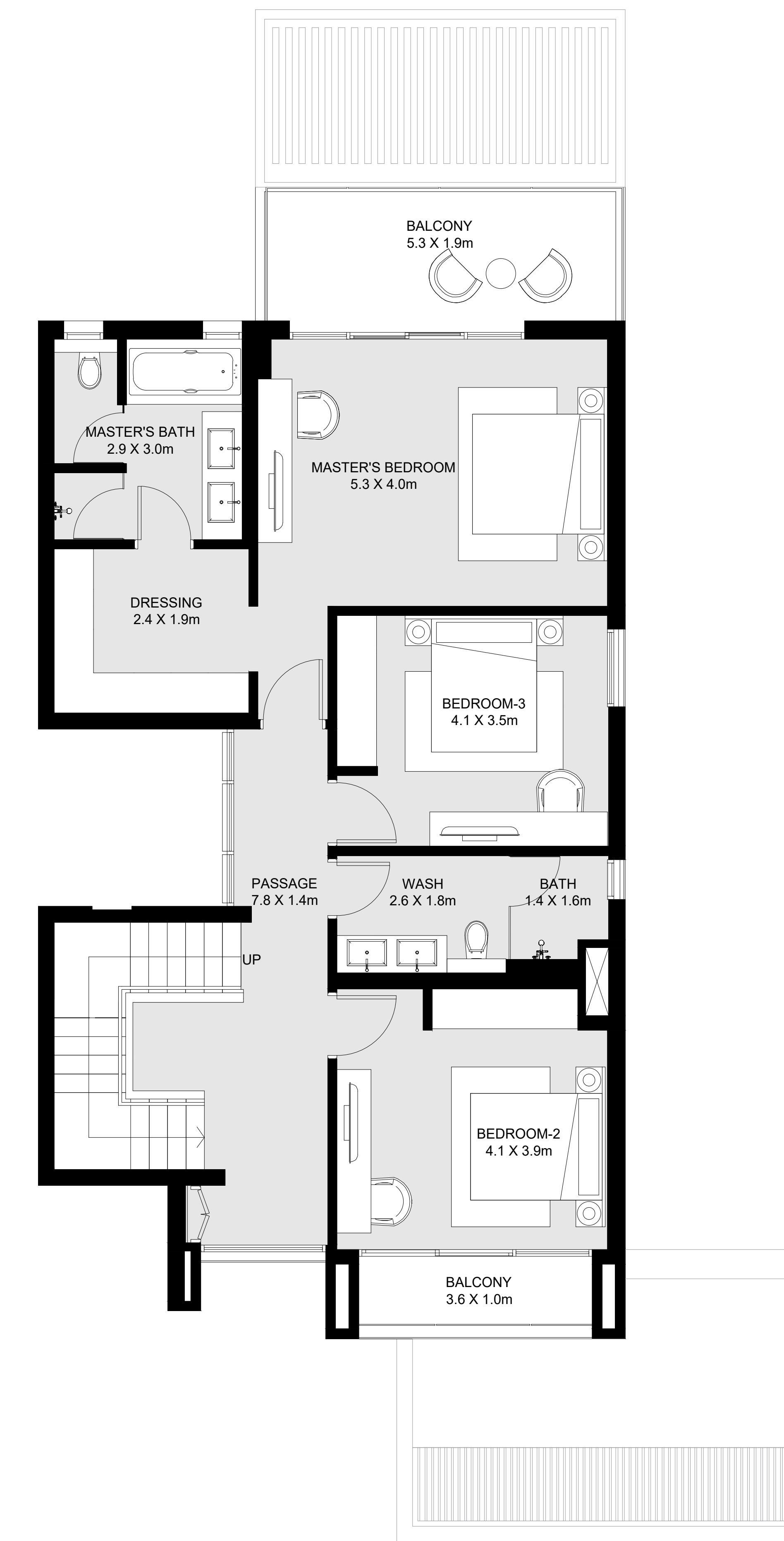
FIRST FLOOR
